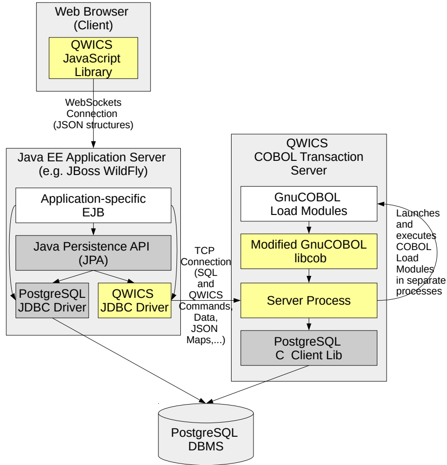
Fig. 1. Overview of the software architecture of QWICS. The arrows denote usage/in-vocation relationships. Yellow boxes describe the QWICS-specific components and white boxes the application-specific COBOL or Java code. The integration between the Java and the COBOL code is achieved using a specific JDBC driver calling the COBOL server via its own protocol over a TCP connection. Reprinted from [6].
