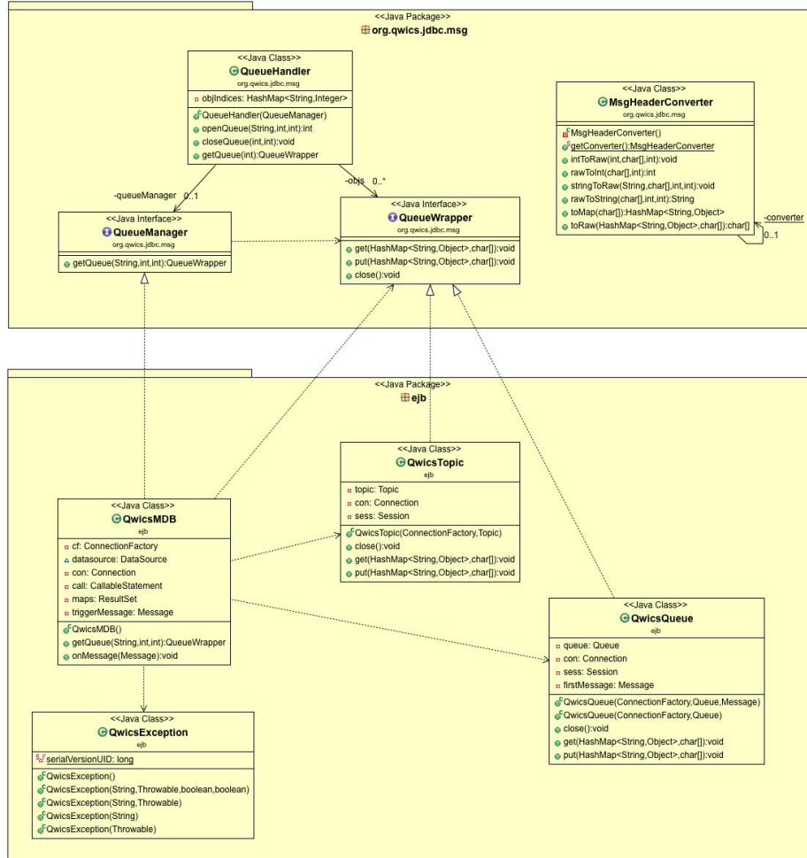
Fig.6. UML class diagram describing the Java-side implementation of an example Message-Driven Bean ( QwicsMDB ) using the newly added message-queueing functionality of the QWICS JDBC driver. The MDB class listens for and reacts to received messages from a JMS queue or topic and provides the driver with appropriate QueueWrapper implementation classes (labeled QwicsQueue and QwicsTopic here) for accessing the respective JMS objects.
