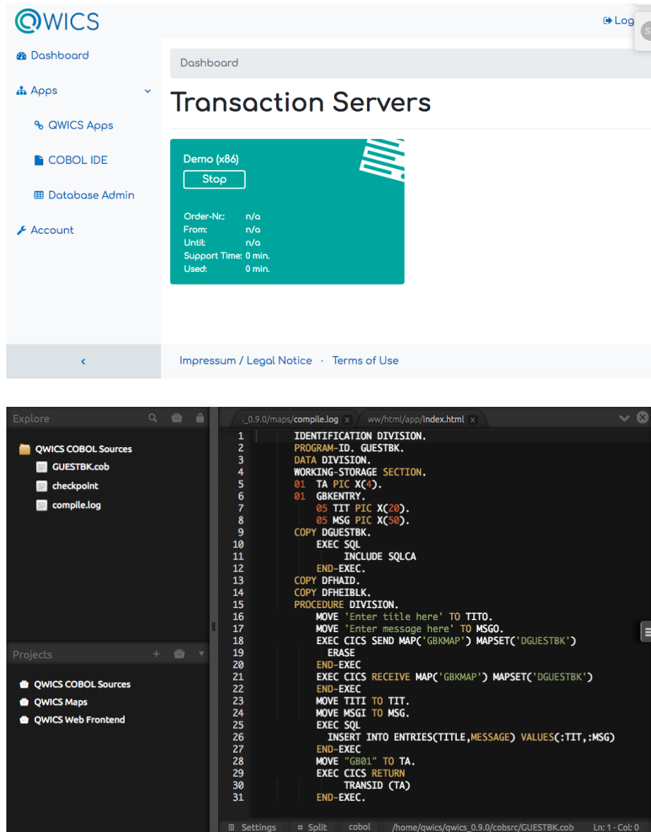
Fig. 9. Screenshots from the free QWICS online demonstration and testing environment: Admin Dashboard showing a running QWICS VM instance (above) and the online source code editor showing a COBOL example (below).
